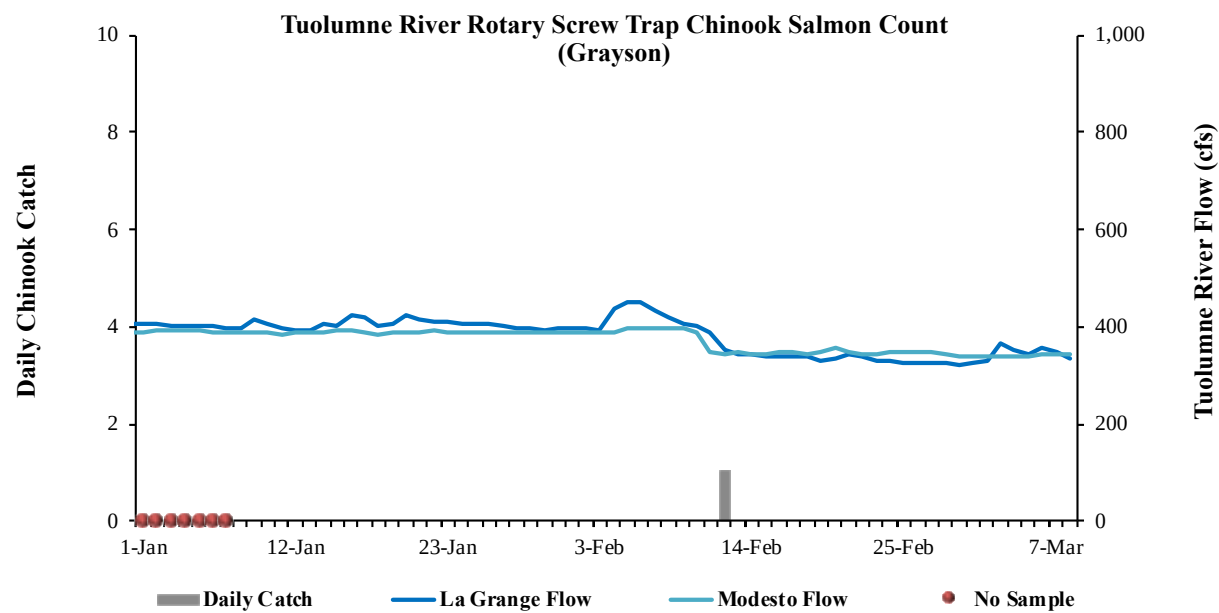
Figure 2. Daily Chinook catch at Grayson RST and Tuolumne River flow at La Grange and Modesto.
