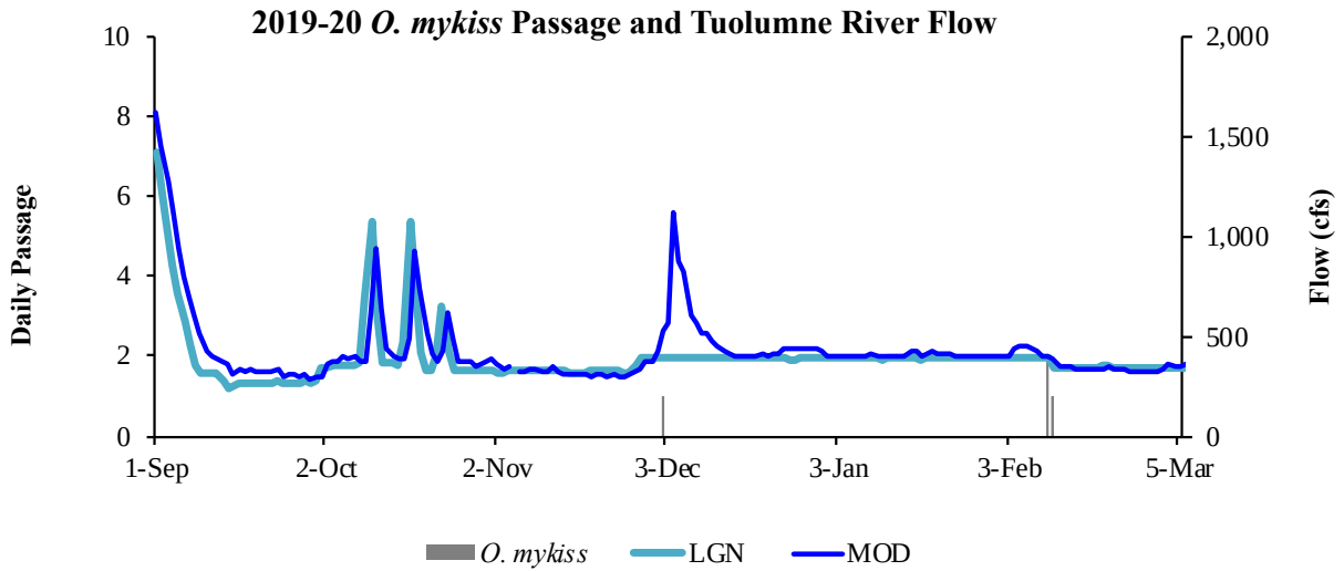
Figure 5. Daily O. mykiss passage at the Tuolumne River weir and river flow at La Grange and Modesto. A net total of four O. mykiss have been detected at the weir since December 2 (all less than 16 inches in length).
