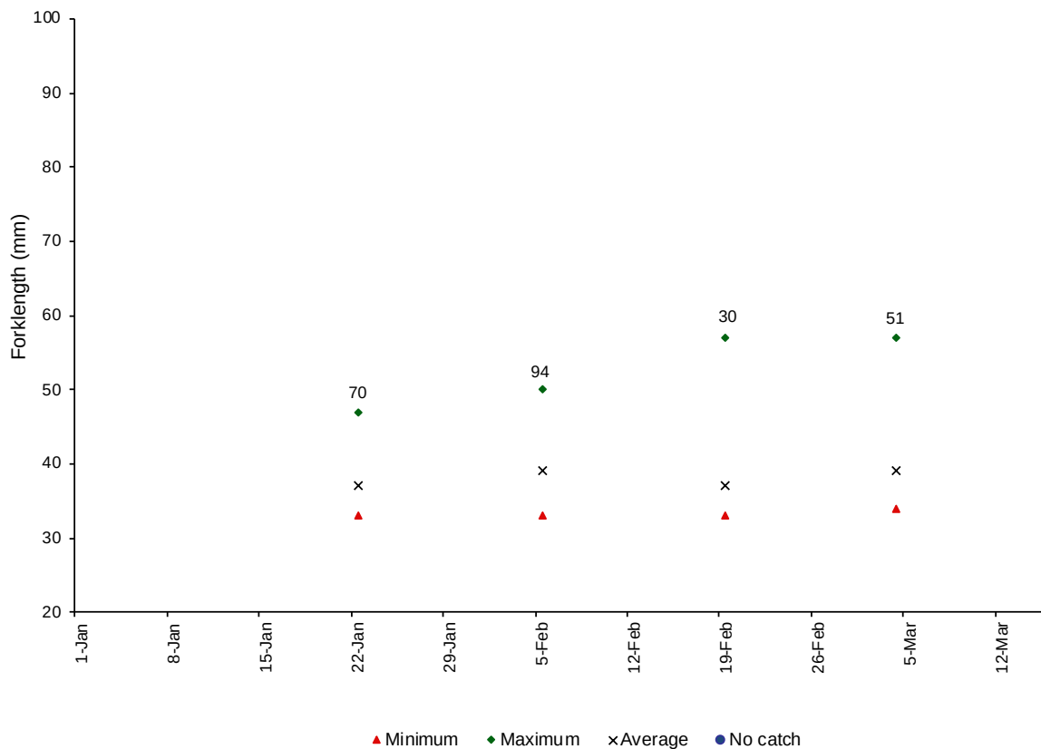
Figure 6. Minimum, maximum and average forklength of Chinook captured in Tuolumne River seine surveys. The number of salmon captured is indicated above the forklength range.
