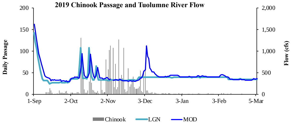
Figure 3. Daily adult Chinook passage at the Tuolumne River weir and river flow at La Grange and Modesto. A total of 2,136 Chinook were counted at the weir through March 5, 2020.
