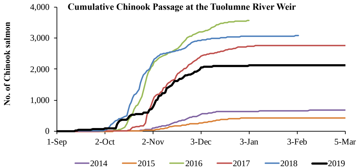
Figure 4. Cumulative daily Chinook passage at the Tuolumne River weir, 2014-2019.
