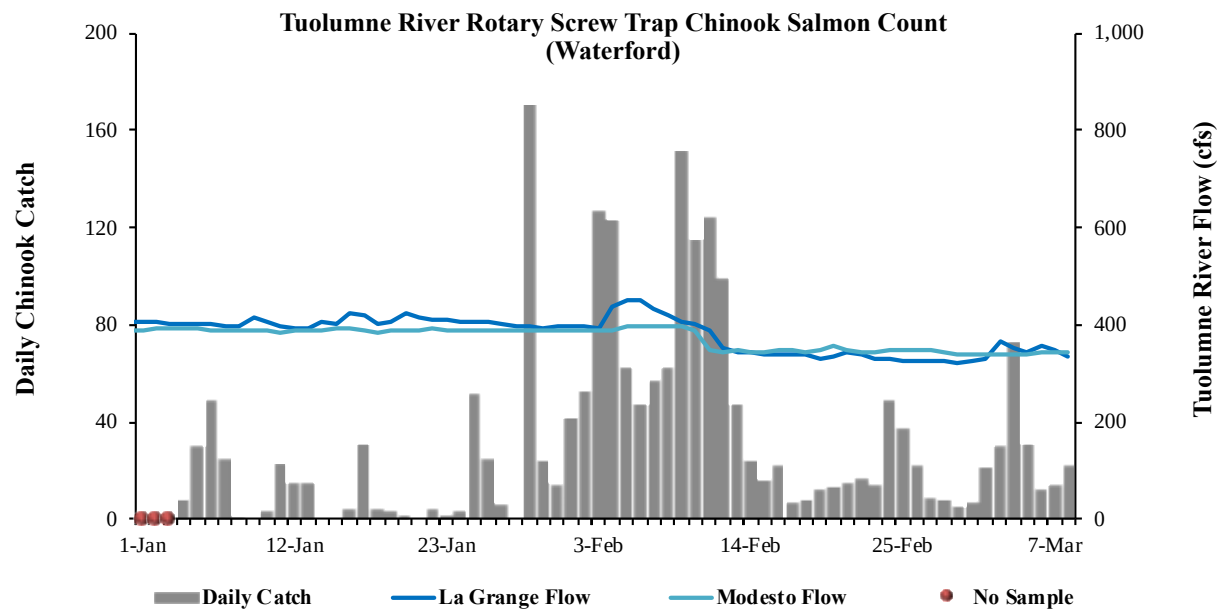
Figure 1. Daily Chinook catch at Waterford RST and Tuolumne River flow at La Grange and Modesto.
